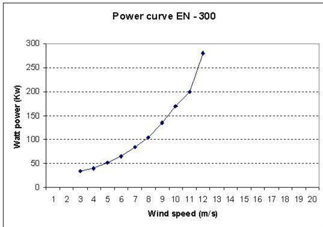
Power curve
